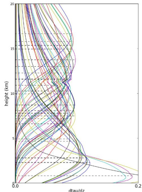
AIRS Weighting Functions: Assimilated Low-peaking T-channels
