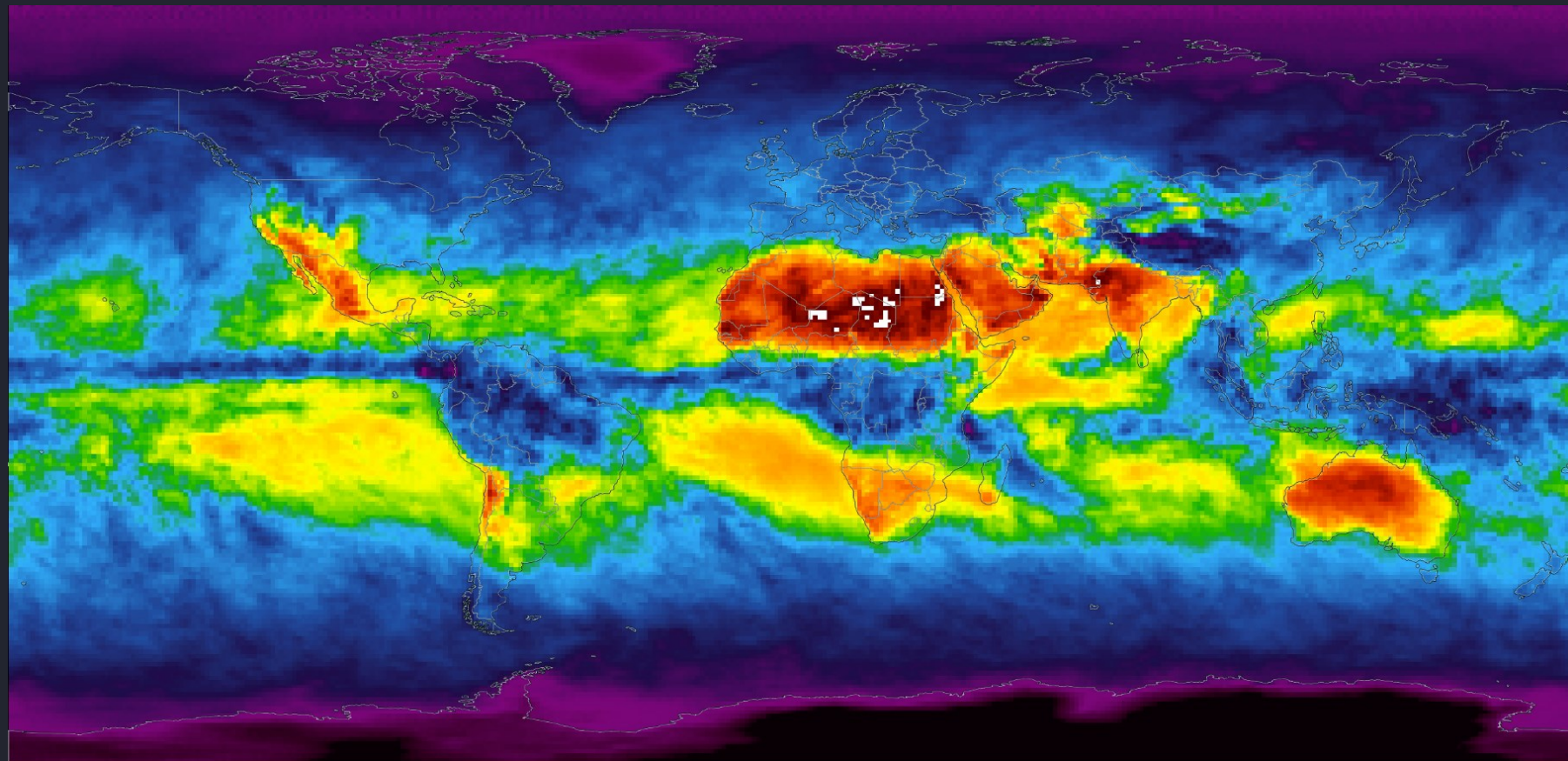
Outgoing Longwave Radiation (L3, Day, Monthly), NASA EOS Worldview
