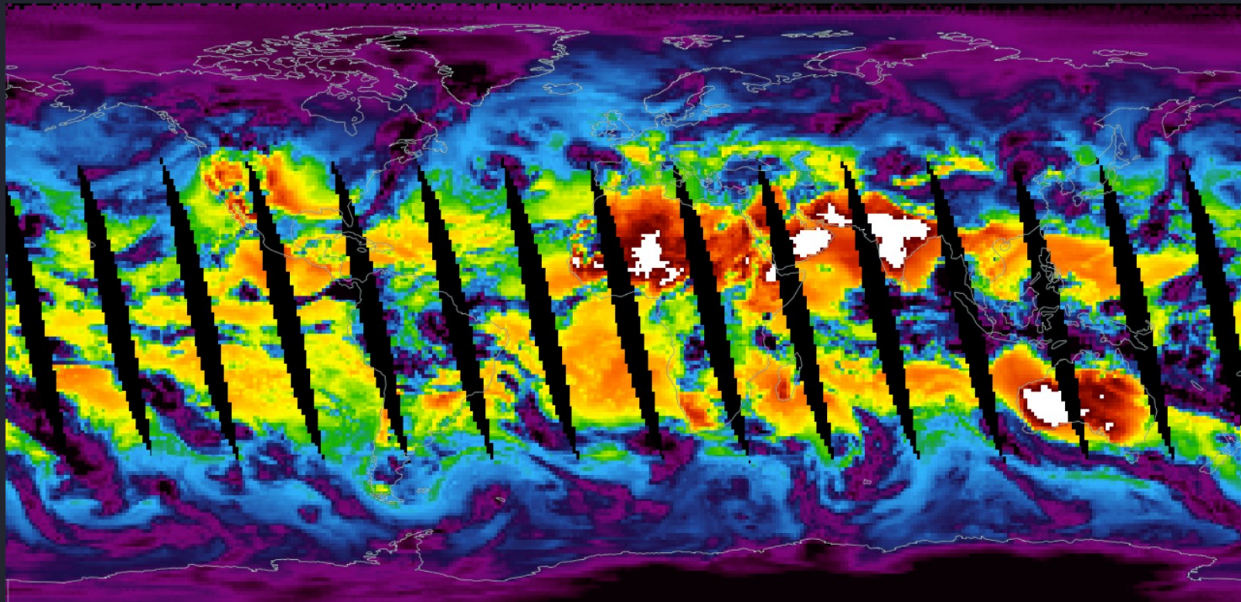
Outgoing Longwave Radiation (L3, Day, Daily), NASA EOS Worldview
