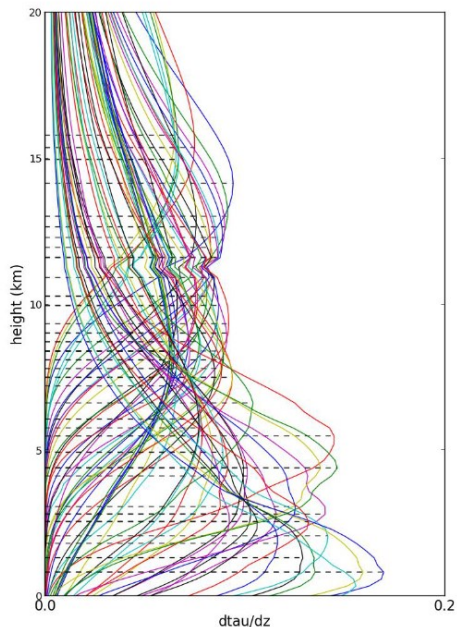
IASI Weighting Functions: Assimilated Low-peaking T-channels
