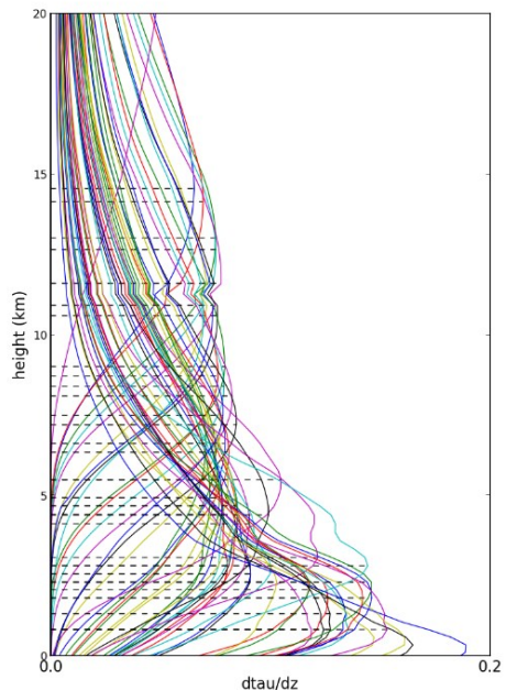
CrIS Weighting Functions: Assimilated Low-peaking T-channels
